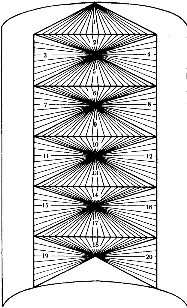
FIGURE 5-9. A surface containing 20 triangles inscribed in a portion of a cylinder. If the number of triangles is increased sufficiently, by making the bases of triangles 3, 4, 7, 8, etc., sufficiently small, the total area of the inscribed surface can be made as large as desired.
